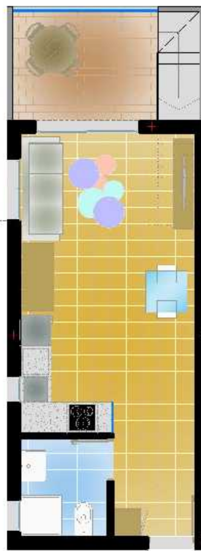
Planta alta / First floor Escala 1/75
